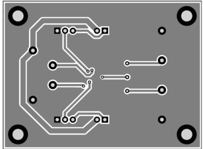
Figure 3: AAT3244 Evaluation Board Bottom Side Layout.
