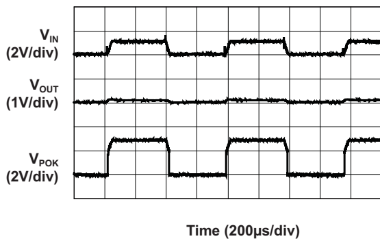
POK Output Response
