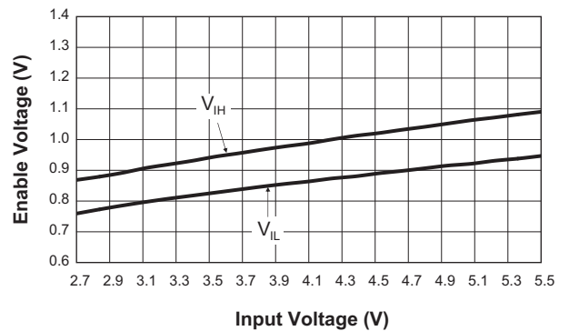
Enable Threshold Voltage vs. Input Voltage
