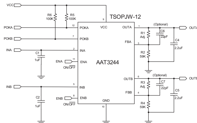
Figure 1: AAT3244 Schematic.
